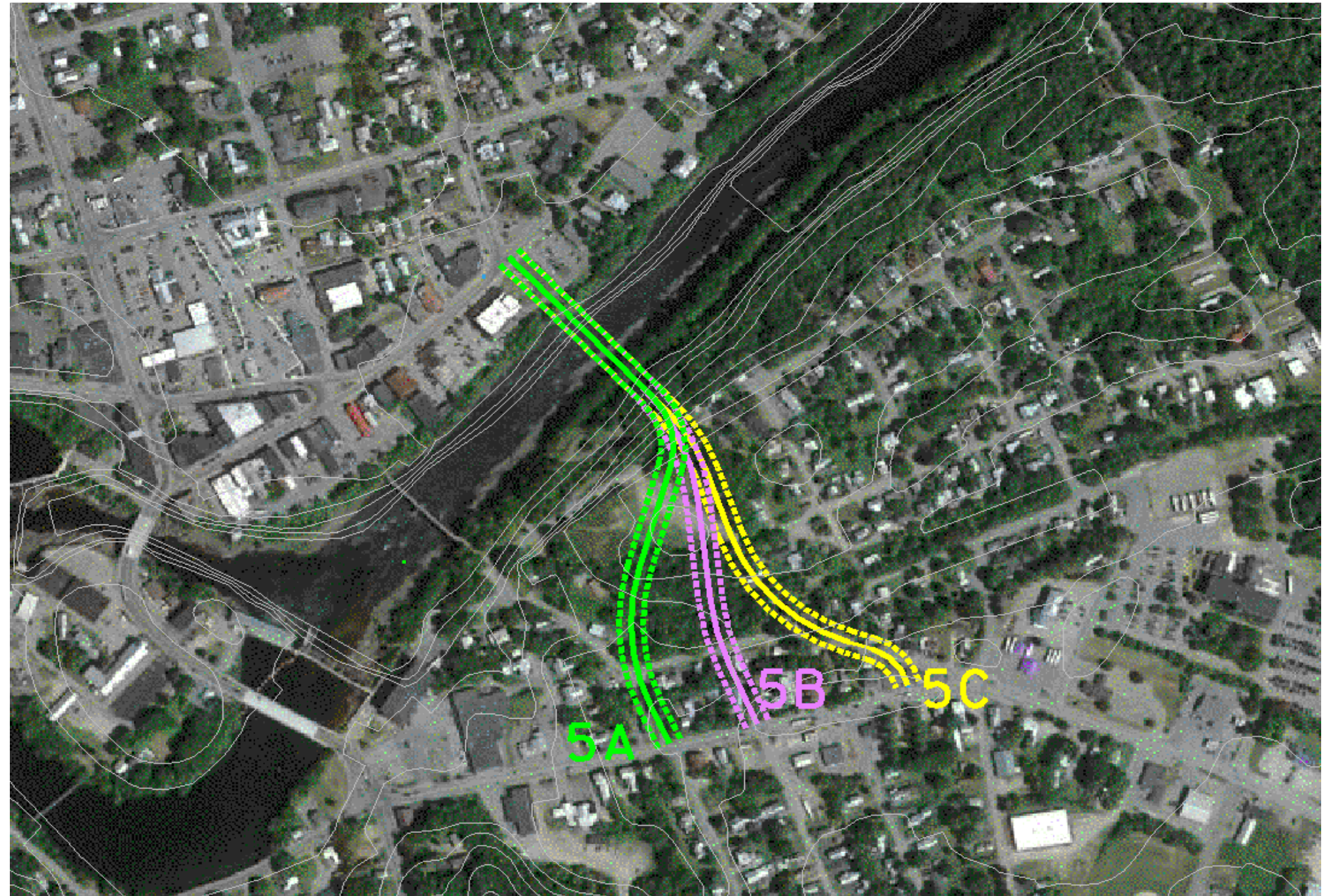
Figure 6.2 – A5 Downtown Bridge Crossing Concept
